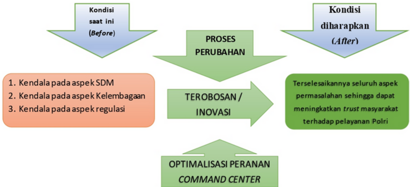
GAMBAR 1 DIAGNOSA GAP
